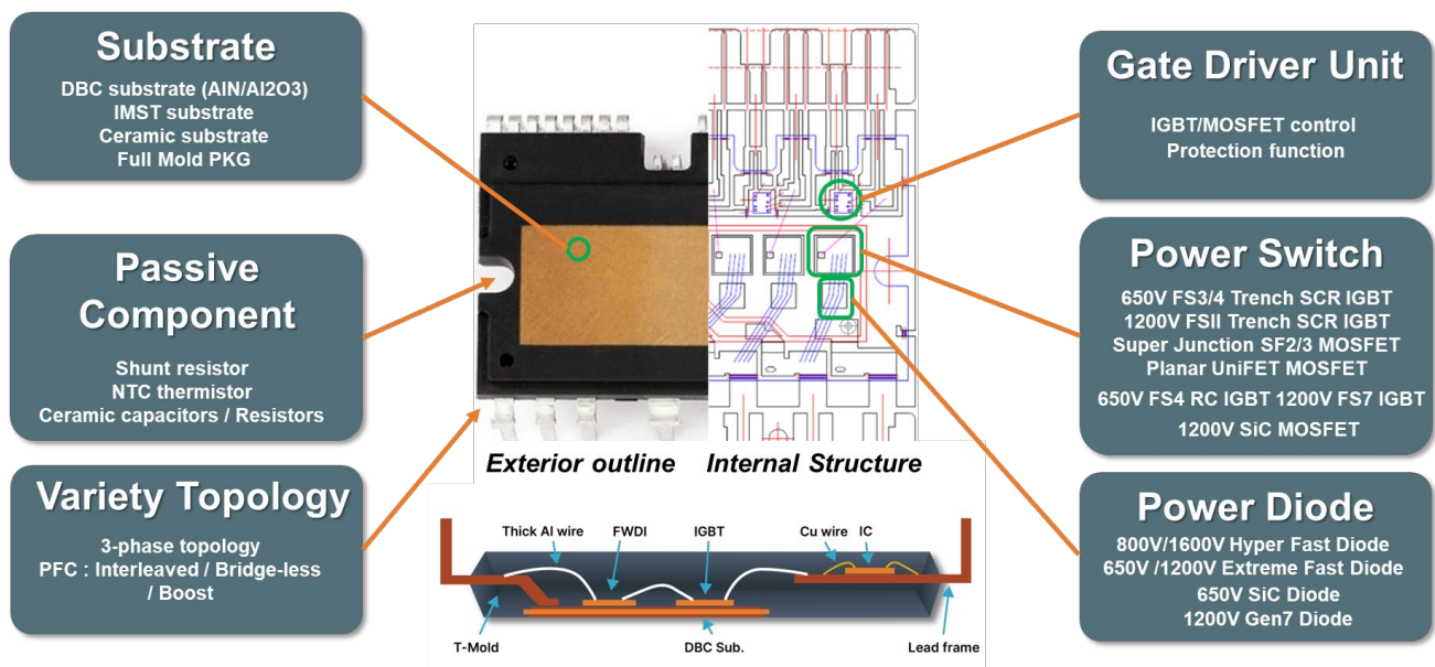
Fig.19: Level of integration of onsemi Intelligent power module
