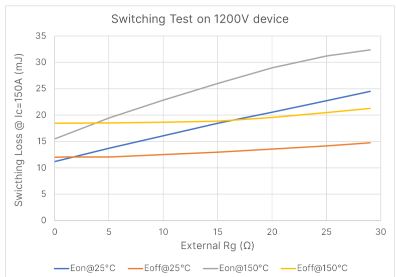
Fig.22: Switching losses of 1200V IGBT from FS7 family
