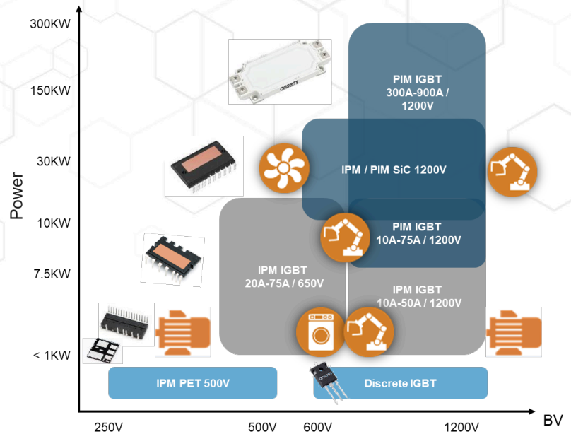
Fig.18: Recommended inverter solution depending on the desired power level and bus voltage
