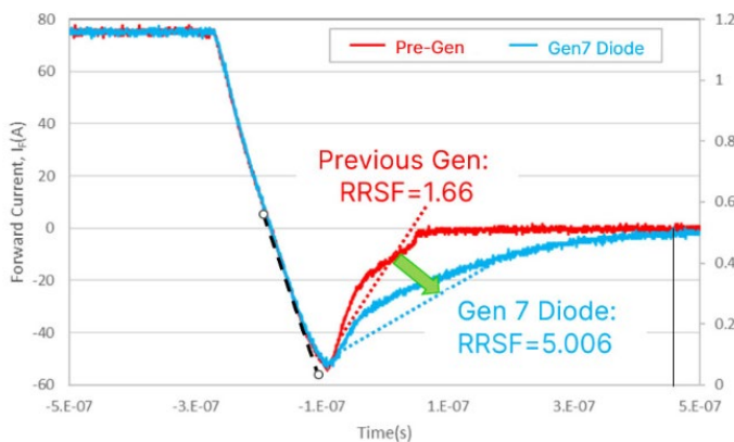
Fig.20: Comparison of softness of Gen7 and previous Gen diode
