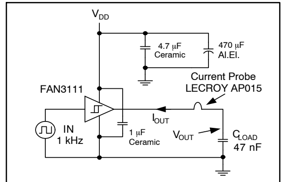
Figure 32. Quasi-Static I_{OUT}/V_{OUT} Test Circuit
