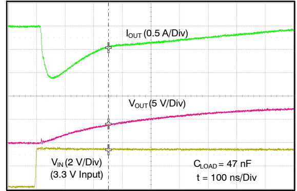
Figure 30. Quasi-Static Source Current ( V_{DD} = 8\text{ V} )
