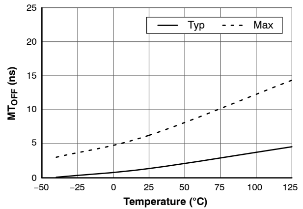
Figure 31. Delay Matching HO and LO Turn-off vs. Temperature
