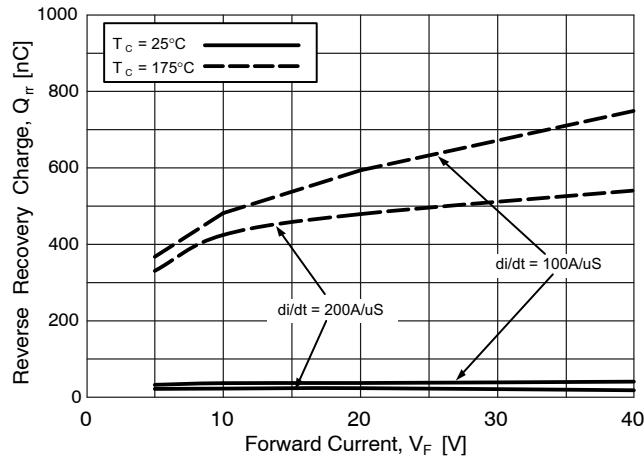
Figure 19. Stored Charge
