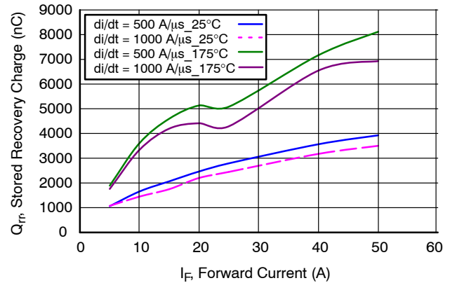
Figure 18. Stored Charge
